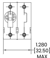
2-POLE (HB2)
