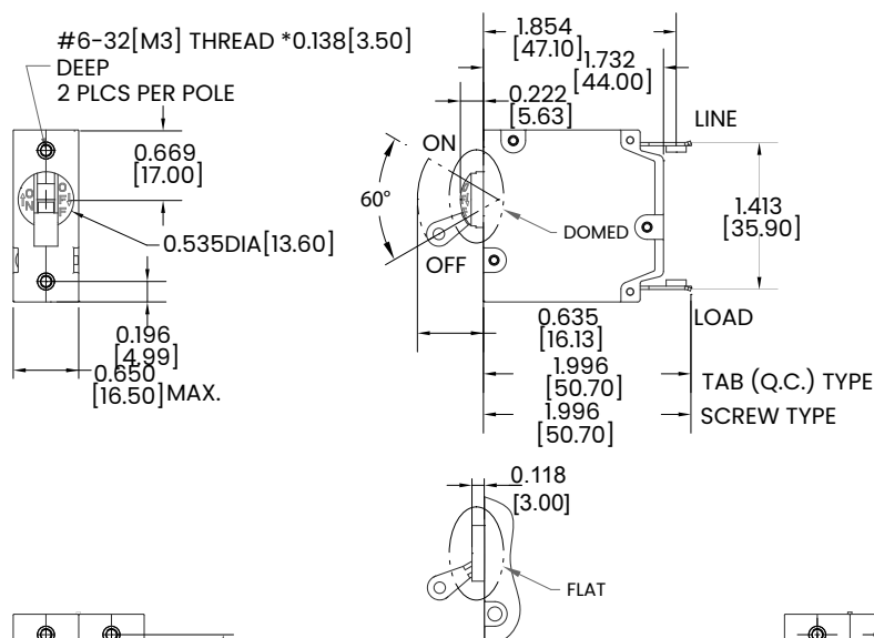
2-POLE (HB2)
