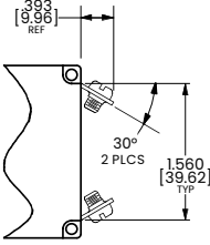
SCREW TERMINAL WITH 30° BEND
