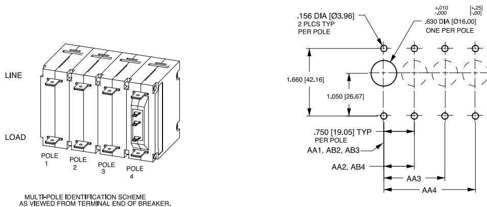
PANEL CUTOUT DETAIL TOLERANCES \pm .005 [ \pm .12 ] UNLESS OTHERWISE SPECIFIED
