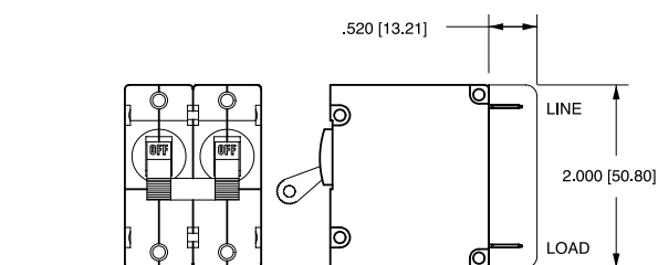
BARRIER FOR UL-RECOGNIZED MULTI-POLE BREAKERS
