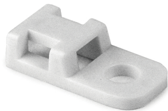
Cable Tie Anchor Mount, 0.17" Hole Dia, 0.20" Max Tie Width, PA66, White, 1000/pkg
