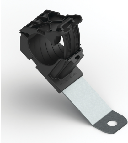
Ratchet P-Clamp, 0.76 - 1.42" Bundle Dia, 30° Long, 0.51" Hole Dia, PA66HIRHSUV/ST/ZN, Black, 140/ctn
