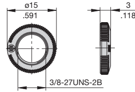
Knurled nut 3/8" plastic (standard) Y 307 117 02
