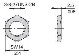
Hex nut 3/8" nickel-plated brass Y 300 192 01
