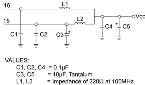
Figure 2 Shows the suggested layout for power and ground connections.
