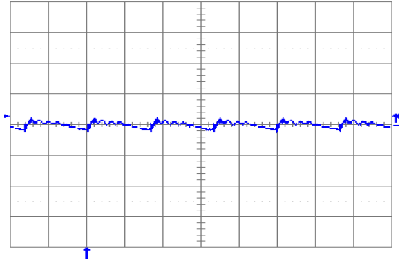
Fig. 1.0V.6: Output voltage ripple (20 mV/div.) at full rated load current into a resistive load with external capacitance 100\text{ }\mu\text{F} ceramic + 1\text{ }\mu\text{F} ceramic, and V_{in} = 12 V for V_{out} = 1.0 V. Time scale: 2 \mu\text{s} /div.
