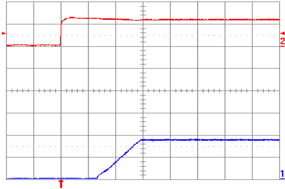
Fig. 1.8V.5: Turn-on transient for V_{out} = 1.8\text{ V} with application of V_{in} at full rated load current (resistive) and 100\text{ }\mu\text{F} external capacitance at V_{in} = 12\text{ V} . Top trace: V_{in} ( 10\text{ V/div.} ); Bottom trace: output voltage ( 1\text{ V/div.} ); Time scale: 2\text{ ms/div.}
