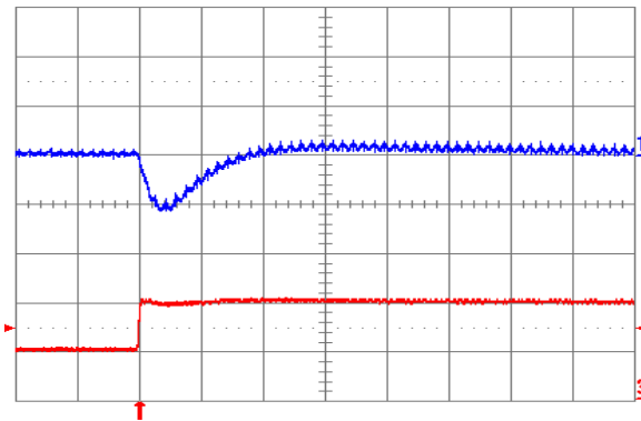
Fig. 1.0V.7: Output voltage response for V_{out} = 1.0 V to positive load current step change from 5 A to 10 A with slew rate of 5\text{ A}/\mu\text{s} at V_{in} = 12 V. Top trace: output voltage (100 mV/div.); Bottom trace: load current (5 A/div.). C_o = 100\text{ }\mu\text{F} ceramic. Time scale: 20 \mu\text{s} /div.
