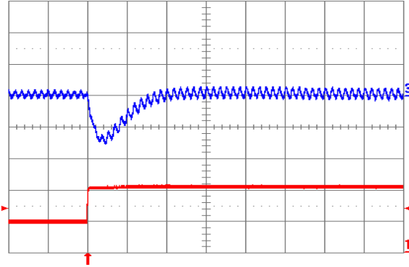
Fig. 5.0V.7: Output voltage response for V_{out} = 5.0\text{ V} to positive load current step change from 5 A to 10 A with slew rate of 5 A/ \mu\text{s} at V_{in} = 12\text{ V} . Top trace: output voltage (100 mV/div.); Bottom trace: load current (5 A/div.). C_o = 100\text{ }\mu\text{F} ceramic. Time scale: 20 \mu\text{s} /div.
