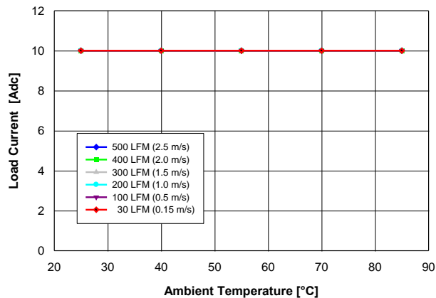
Fig. 1.8V.1: Available load current vs. ambient temperature and airflow rates for V_{out} = 1.8\text{ V} converter mounted vertically with V_{in} = 12\text{ V} , and maximum MOSFET temperature \leq 110\text{ }^{\circ}\text{C} .
