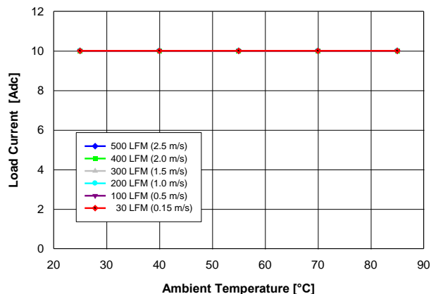
Fig. 0.7525V.1: Available load current vs. ambient temperature and airflow rates for V_{out} = 0.7525 V converter mounted vertically with V_{in} = 12 V, and maximum MOSFET temperature \leq 110\text{ }^{\circ}\text{C} .
