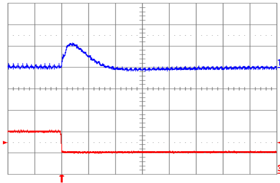
Fig. 1.0V.8: Output voltage response for V_{out} = 1.0 V to negative load current step change from 10 A to 5 A with slew rate of -5\text{ A}/\mu\text{s} at V_{in} = 12 V. Top trace: output voltage (100 mV/div.); Bottom trace: load current (5 A/div.). C_o = 100\text{ }\mu\text{F} ceramic. Time scale: 20 \mu\text{s} /div.
