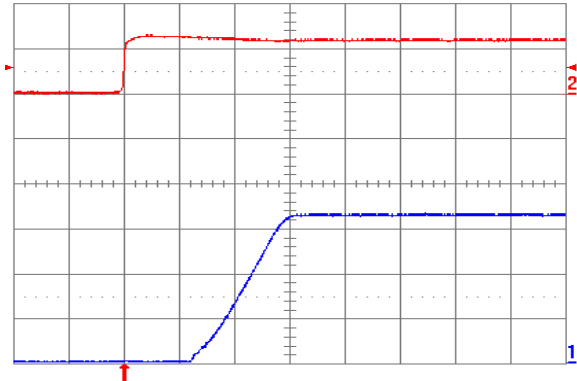
Fig. 3.3V.5: Turn-on transient for V_{out} = 3.3\text{ V} with application of V_{in} at full rated load current (resistive) and 100\text{ }\mu\text{F} external capacitance at V_{in} = 12\text{ V} . Top trace: V_{in} ( 10\text{ V/div.} ); Bottom trace: output voltage ( 1\text{ V/div.} ); Time scale: 2\text{ ms/div.}
