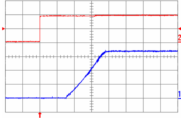
Fig. 0.7525V.5: Turn-on transient for V_{out} = 0.7525 V with the application of Enable signal at full rated load current (resistive) and 100\text{ }\mu\text{F} external capacitance at V_{in} = 5 V. Top trace: Enable signal (2 V/div.); Bottom trace: output voltage (200 mV/div.); Time scale: 2 ms/div.
