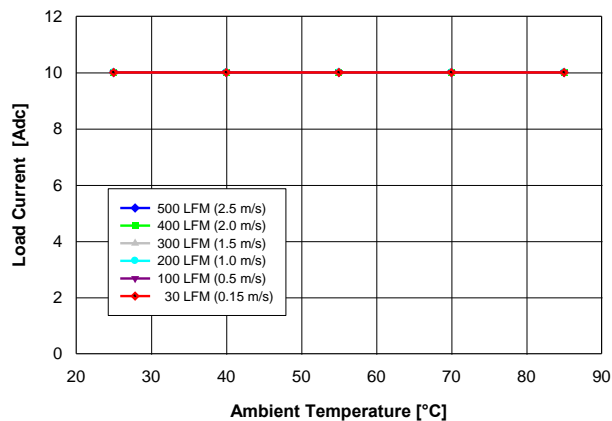
Fig. 1.2V.1: Available load current vs. ambient temperature and airflow rates for V_{out} = 1.2 V converter mounted vertically with V_{in} = 5 V, and maximum MOSFET temperature \leq 120\text{ }^{\circ}\text{C} .
