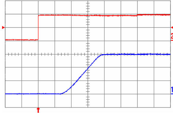
Fig. 1.5V.5: Turn-on transient for V_{out} = 1.5 V with the application of Enable signal at full rated load current (resistive) and 100\text{ }\mu\text{F} external capacitance at V_{in} = 5 V. Top trace: Enable signal (2 V/div.); Bottom trace: output voltage (500 mV/div.); Time scale: 2 ms/div.
