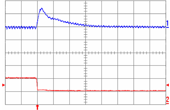
Fig. 1.0V.8: Output voltage response for V_{out} = 1.0 V to negative load current step change from 10 A to 5 A with slew rate of -5 A/μs at V_{in} = 5 V. Top trace: output voltage (100 mV/div.); Bottom trace: load current (5 A/div.). C_o = 100 μF ceramic + 1 μF ceramic. Time scale: 20 μs/div.
