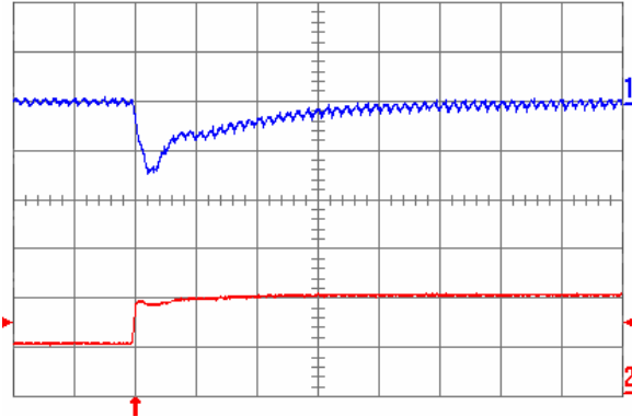
Fig. 1.0V.7: Output voltage response V_{out} = 1.0 V to positive load current step change from 5 A to 10 A with slew rate of 5 A/μs at V_{in} = 5 V. Top trace: output voltage (100 mV/div.); Bottom trace: load current (5 A/div.). C_o = 100 μF ceramic + 1 μF ceramic. Time scale: 20 μs/div.
