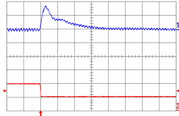
Fig. 1.5V.8: Output voltage response for V_{out} = 1.5 V to negative load current step change from 10 A to 5 A with slew rate of -5\text{ A}/\mu\text{s} at V_{in} = 5 V. Top trace: output voltage (100 mV/div.); Bottom trace: load current (5 A/div.). C_o = 100\text{ }\mu\text{F} ceramic + 1\text{ }\mu\text{F} ceramic. Time scale: 20\text{ }\mu\text{s/div.}
