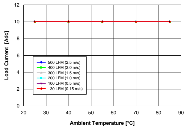
Fig. 1.2V.2: Available load current vs. ambient temperature and airflow rates for V_{out} = 1.2 V converter mounted horizontally with V_{in} = 5 V, and maximum MOSFET temperature \leq 120\text{ }^{\circ}\text{C} .
