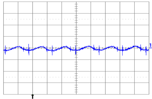
Fig. 2.5V.6: Output voltage ripple (20mV/div.) at full rated load current into a resistive load with external capacitance 100\mu F ceramic and V_{in} = 12V for V_{out} = 2.5V . Time scale: 2µs/div.
