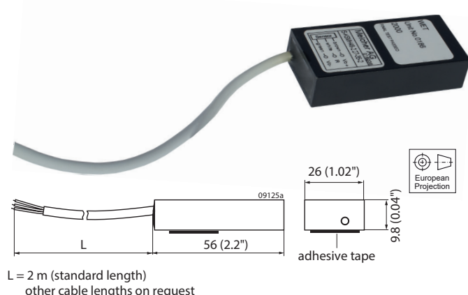
Fig. 25 Temperature sensor
