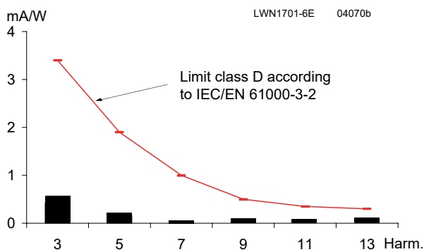
Fig. 4 Harmonic currents at input current, measured at V_i = 230 \text{ VAC} , I_o = I_{o \text{ nom}} (LWN1701-6E).
