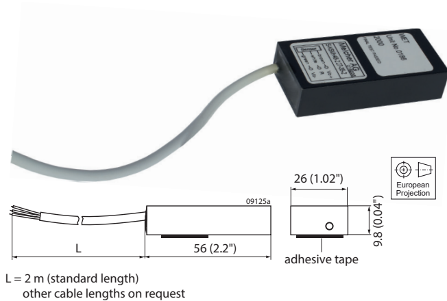
Fig. 26 Temperature sensor
