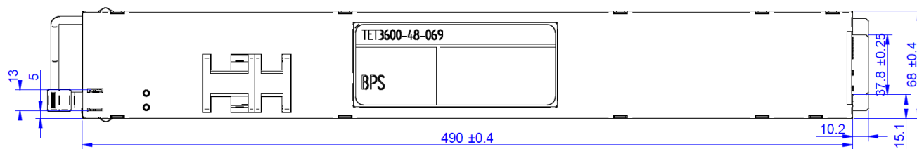
Figure 10. Top view
