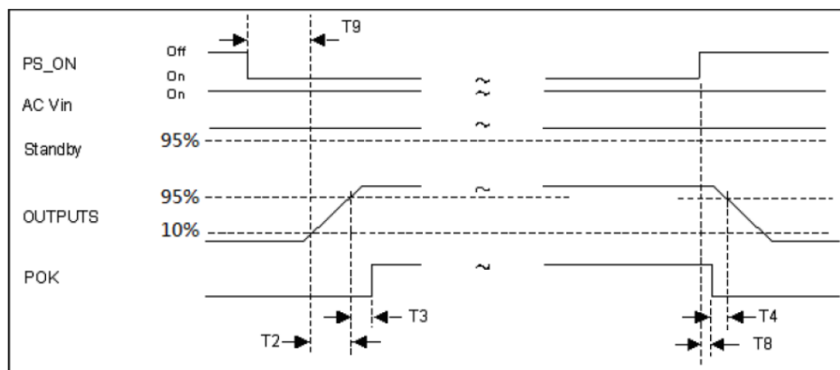
Figure 7. PS_ On/Off Timing
