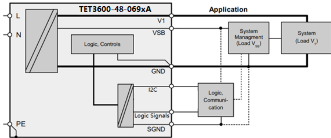
Figure 4. Output connection
