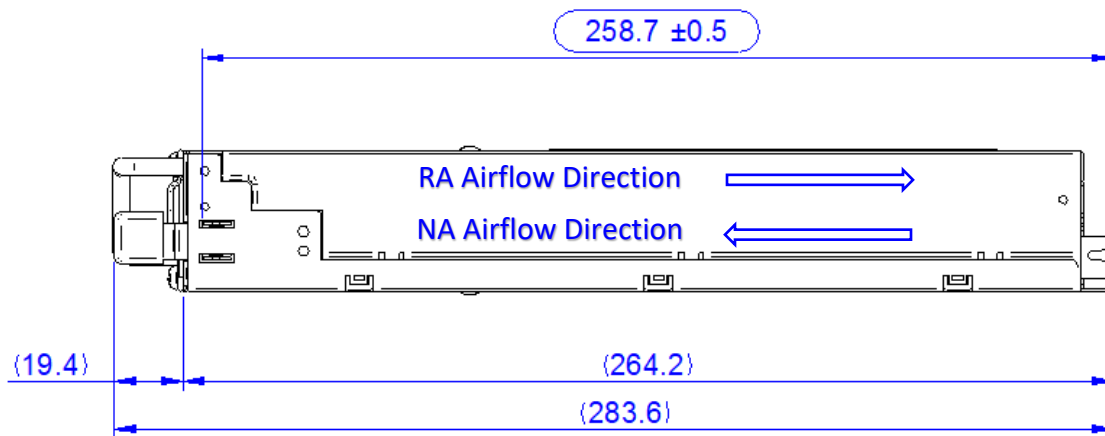
Figure 12. Side view
