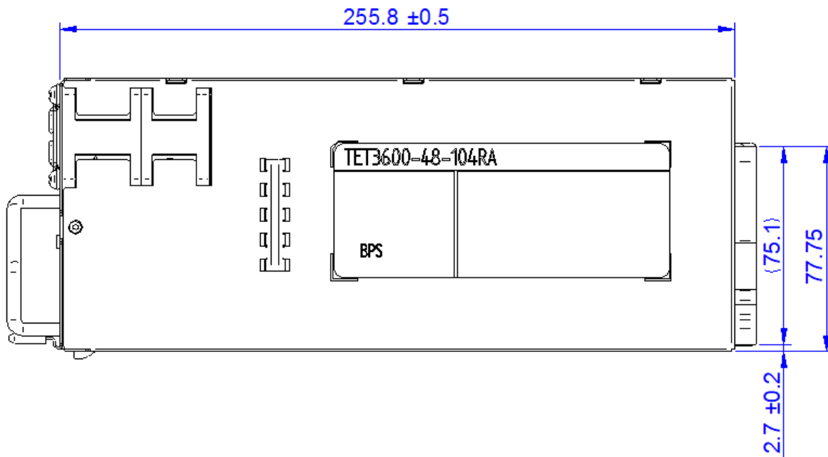
Figure 11. Top view
