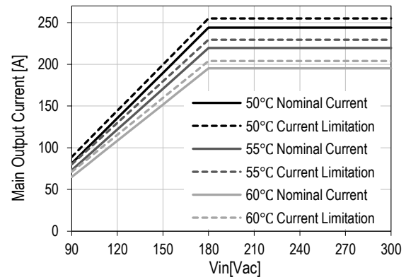
Figure 20. Derating on V_1 vs T_a & V_{in}
