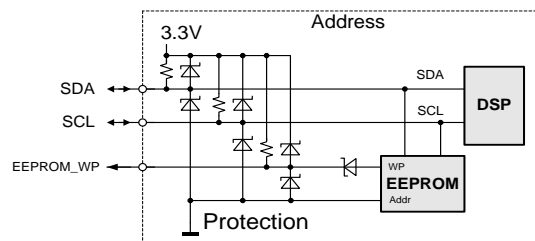
Figure 29. I²C Bus to DSP and EEPROM
