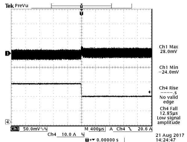
Figure 18. V_{in}=11V , V_o=1.8V , I_o=75\%-50\%I_{o\ max} , di/dt=1A/us
