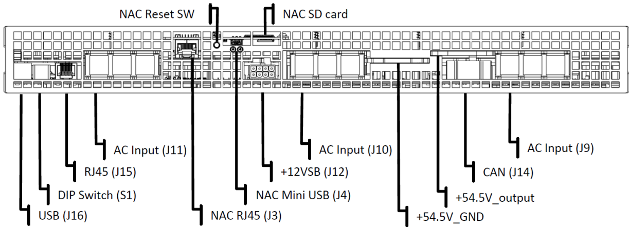
Figure 3. SPSTET4-02 Front View
