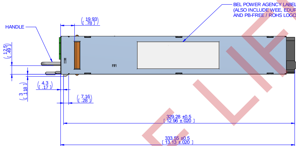
Figure 2. Top View
