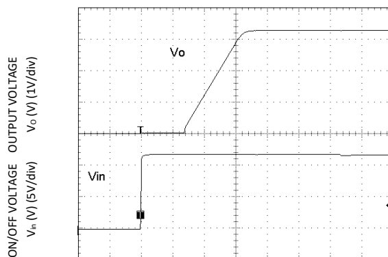
Figure 33. Start-up Using Input Voltage ( V_{IN} = 12V , I_o = I_{o,max} ), V_o = 1.8V
