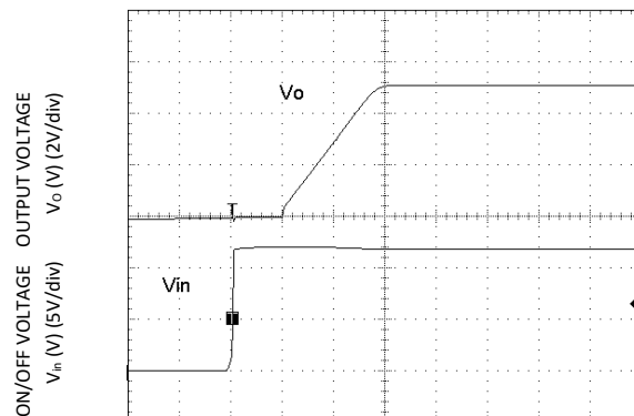
Figure 34. Start-up Using Input Voltage ( V_{IN} = 12V , I_o = I_{o,max} ), V_o = 2.5V
