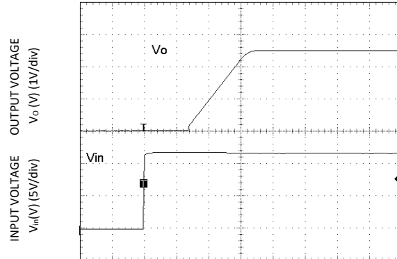
Figure 32. Start-up Using Input Voltage ( V_{IN} = 12V , I_o = I_{o,max} ), V_o = 1.2V
