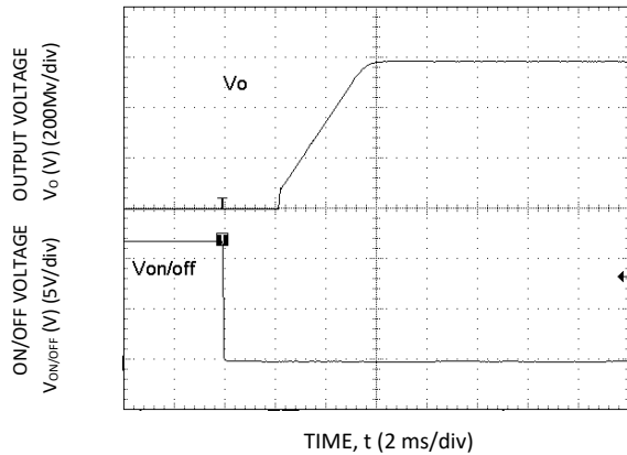
Figure 25. Start-up Using On/Off Voltage ( I_o = I_{o,max} , V_o = 0.6\text{ V} )
