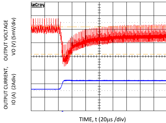
Figure 19. Transient Response to Dynamic Load Change from 50% to 100% at 12V in , C out = 1x 47 \mu F + 4x 330 \mu F, C Tune = 33 nF, R Tune = 178 \Omega . V_o = 0.6\text{ V}
