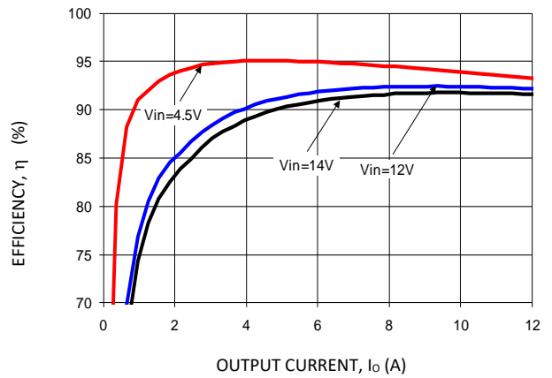
Figure 4. V_o = 2.5\text{ V}
