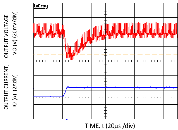
Figure 21. Transient Response to Dynamic Load Change from 50% to 100% at 12V in , C out = 1x 47 \mu F + 1x 330 \mu F, C Tune = 4700 pF, R Tune = 178 \Omega . V_o = 1.8\text{ V}
