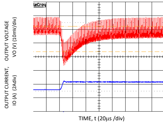
Figure 20. Transient Response to Dynamic Load Change from 50% to 100% at 12V in , C out = 1x 47 \mu F + 2x 330 \mu F, C Tune = 12 nF, R Tune = 178 \Omega . V_o = 1.2\text{ V}
