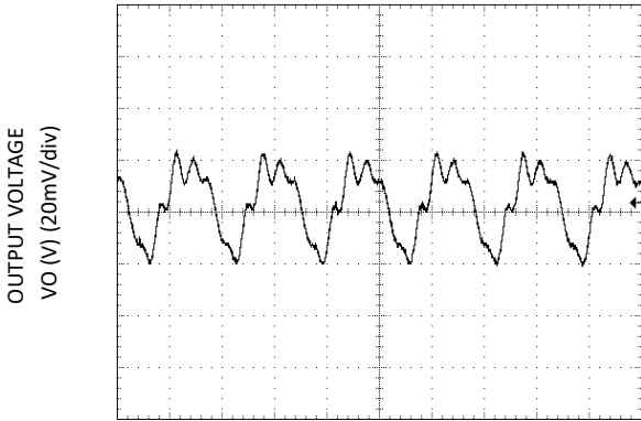
Figure 15. V_o = 1.8\text{ V} , I_o = I_{o,max}
