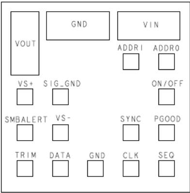
Figure 53. Pins (Bottom View)
