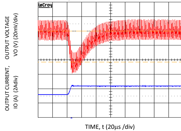
Figure 22. Transient Response to Dynamic Load Change from 50% to 100% at 12V in , C out = 3x 47 \mu F, C Tune = 3300 pF, R Tune = 178 \Omega . V_o = 2.5\text{ V}
