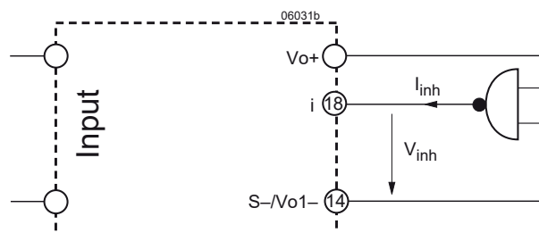
Fig. 17 Definition of V_{inh} and I_{inh} .
