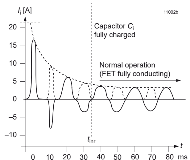
Fig. 33 Typ. inrush current with option E V_i = 230 VAC, f_i = 50 Hz, P_o = P_{o\text{ nom}}
