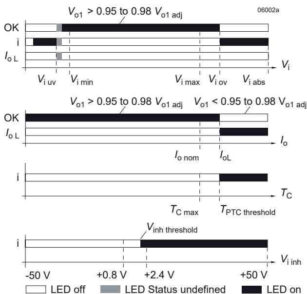
Fig. 22 LED indicators
