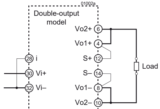
Fig. 2 Parallel-output configuration
