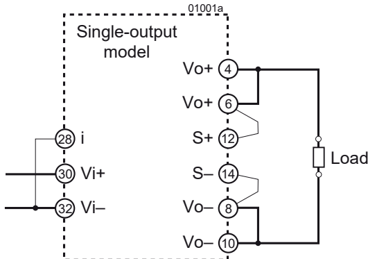
Fig. 1 Single-output configuration
