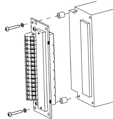
Fig. 24 Cage clamp adapter HZZ00144-G
