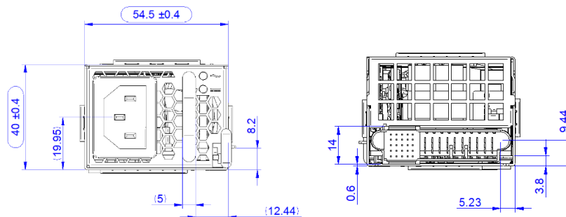
Figure 27. Side View
