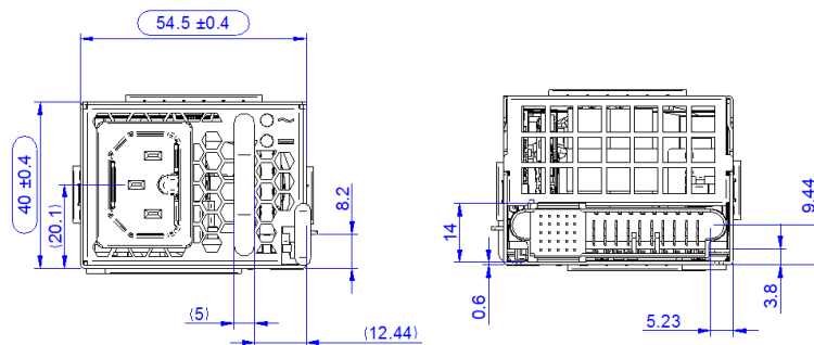
Figure 30. Side View
