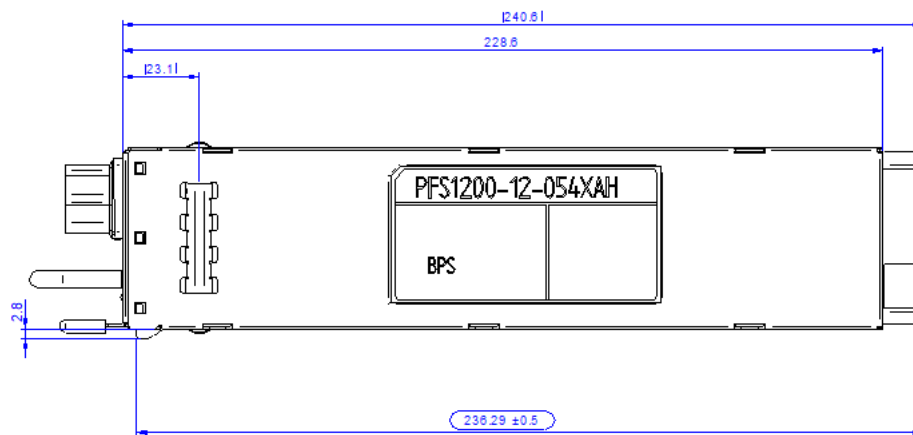
Figure 23. Top View
