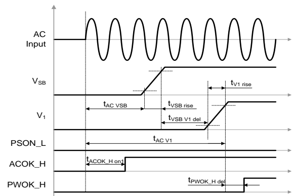
Figure 11. AC turn-on timing
