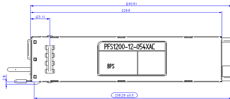
Figure 29. Side View
