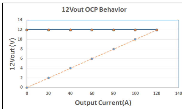
Figure 6a. Current Limitation on V_I ( V_i = 230\text{ VAC} )
