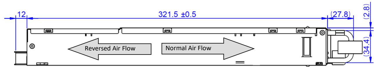
Figure 14 Side View 1
