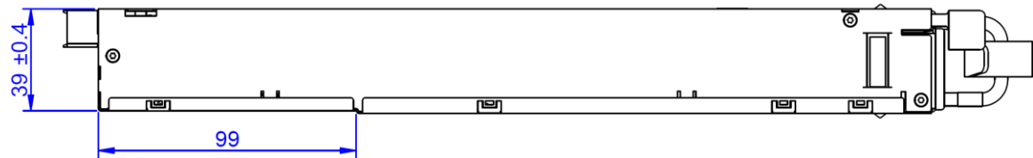
Figure 28. Side View 2
