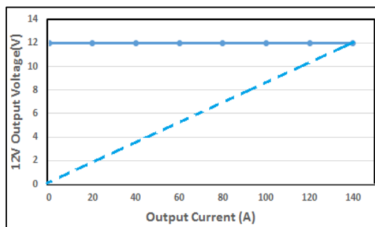
Figure 6. Current Limitation on V_I
