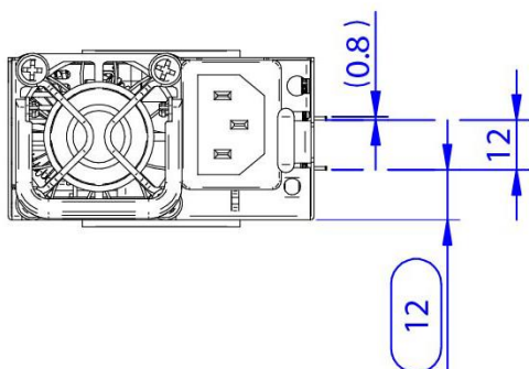
Figure 30. Front view
