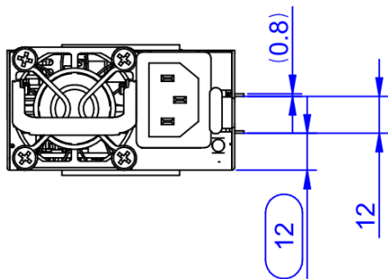
Figure 48. Front view
