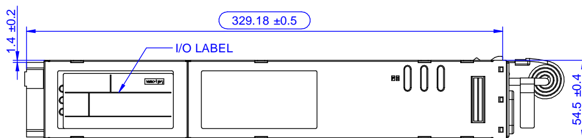
Figure 16. Top View
