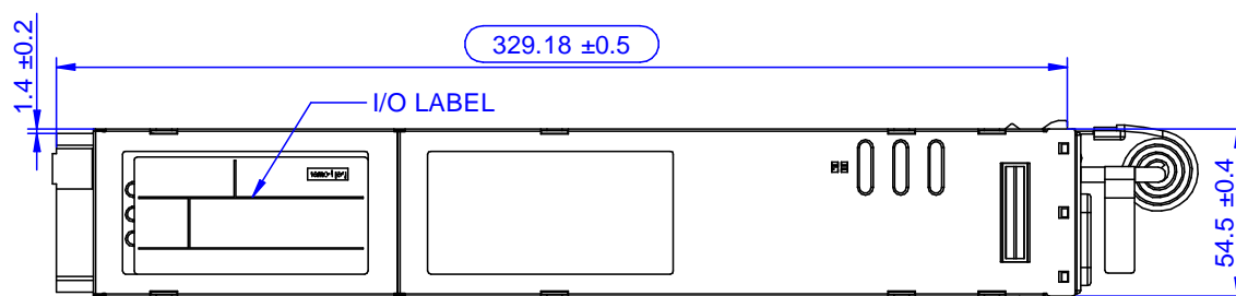
Figure 16. Top View
