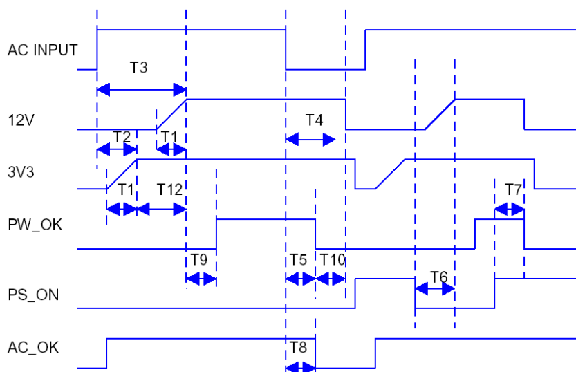
Figure 14. Timing Diagram
