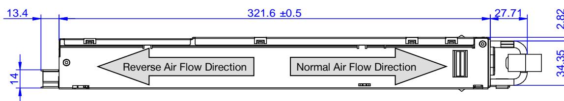
Figure 15. Side View 1
