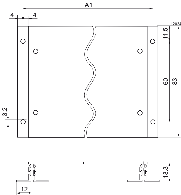
Fig. 10 Dimensions of chassis mounting support (CMB) Bracket: Aluminum, black finish
