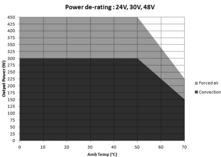
Figure 1. Derating Curves
