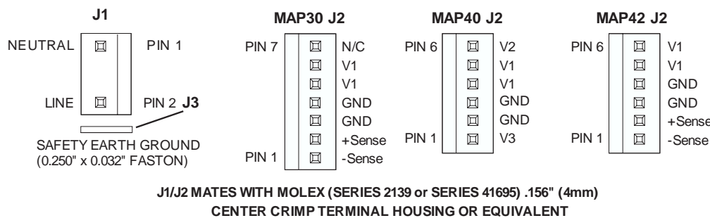
Figure 4. Electrical Connectors
