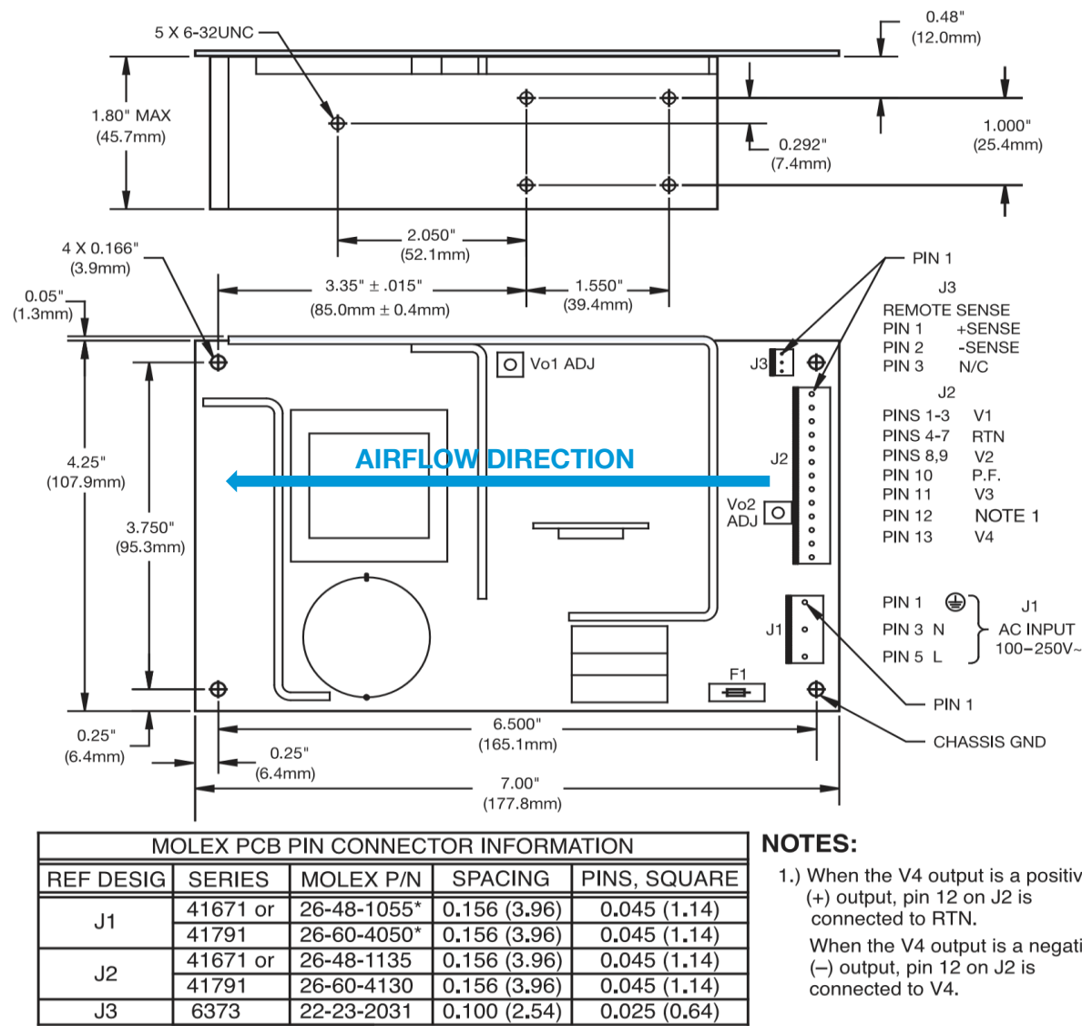
Figure 1. Mechanical Drawing
