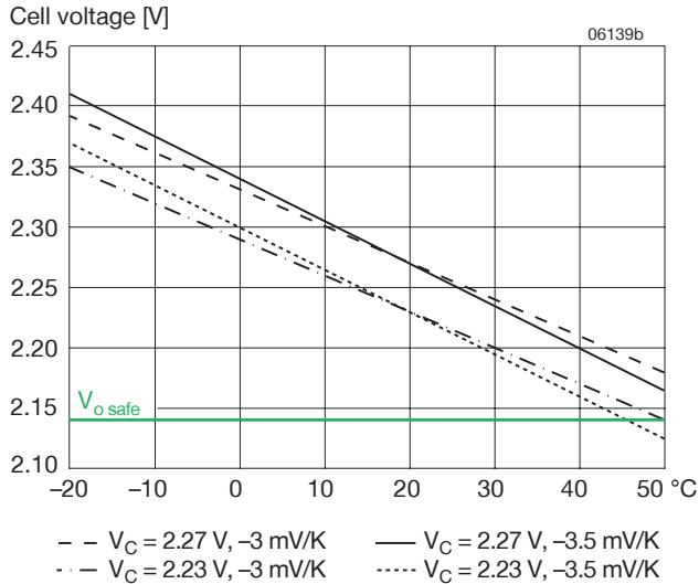
Fig. 16 Trickle charge voltage versus temperature for defined temperature coefficient.
