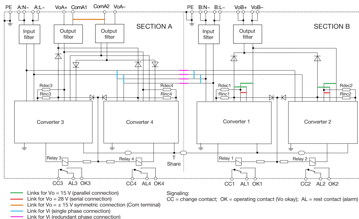
Block diagram of the rack. The converters in the different positions are fitted depending on the configuration; see table 2. Section A & B: The magenta connection is valid for operation on two independent AC input voltages. Cyan connection is valid for operation on one single AC input voltage. Section A: The orange connection is valid for \pm V_o symmetric connection (Com terminal). Section B: The green connections are valid for the parallel configuration with 15 V or 24 V output, the red connections for serial configuration with 28 V, 30 V, 48V or 50 V output. For details of contacts and wires, see Mechanical Data. T Share jumper between sections A and B is fitted on models -900G only.
