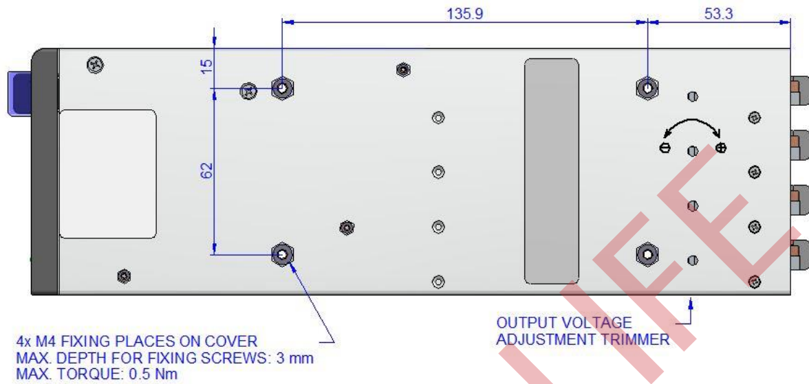
Figure 10. Bottom View
