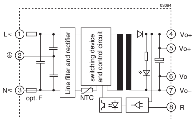
Fig. 1 Block diagram LOK4301, LOK4601 and 4801 (rectifier versions), all LOR and all LOS.
