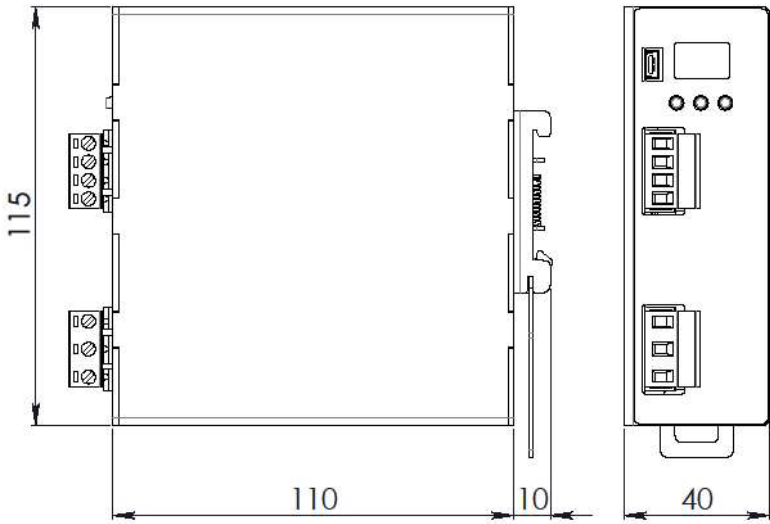
Figure 3. Mechanical Drawing
