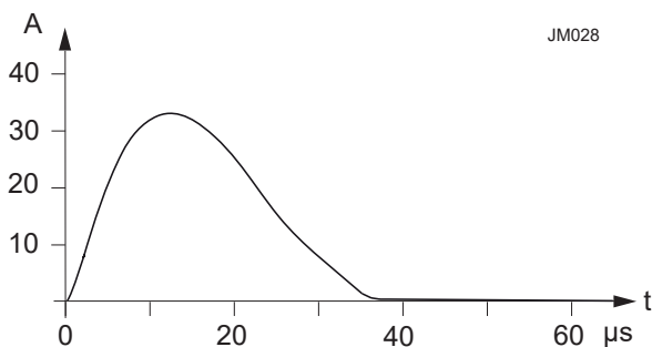
Fig. 3 Inrush current at V_{i\text{ nom}} , P_{o\text{ nom}} versus time (110IMY70-24-24-8). Source impedance according to ETS 300132-2: L = 10\text{ μH} , R = 1.5\text{ Ω} .
