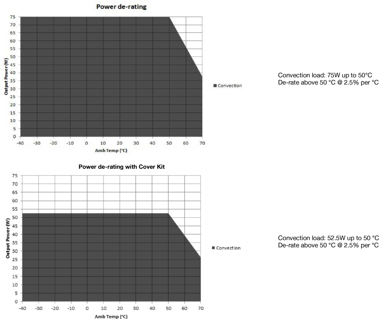
Figure 1. Derating Curves
