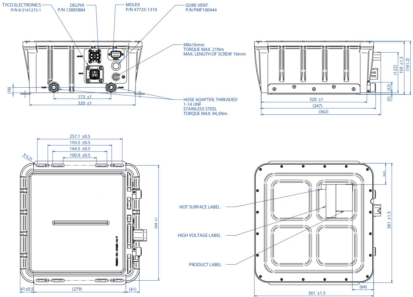
Figure 5. Front view
