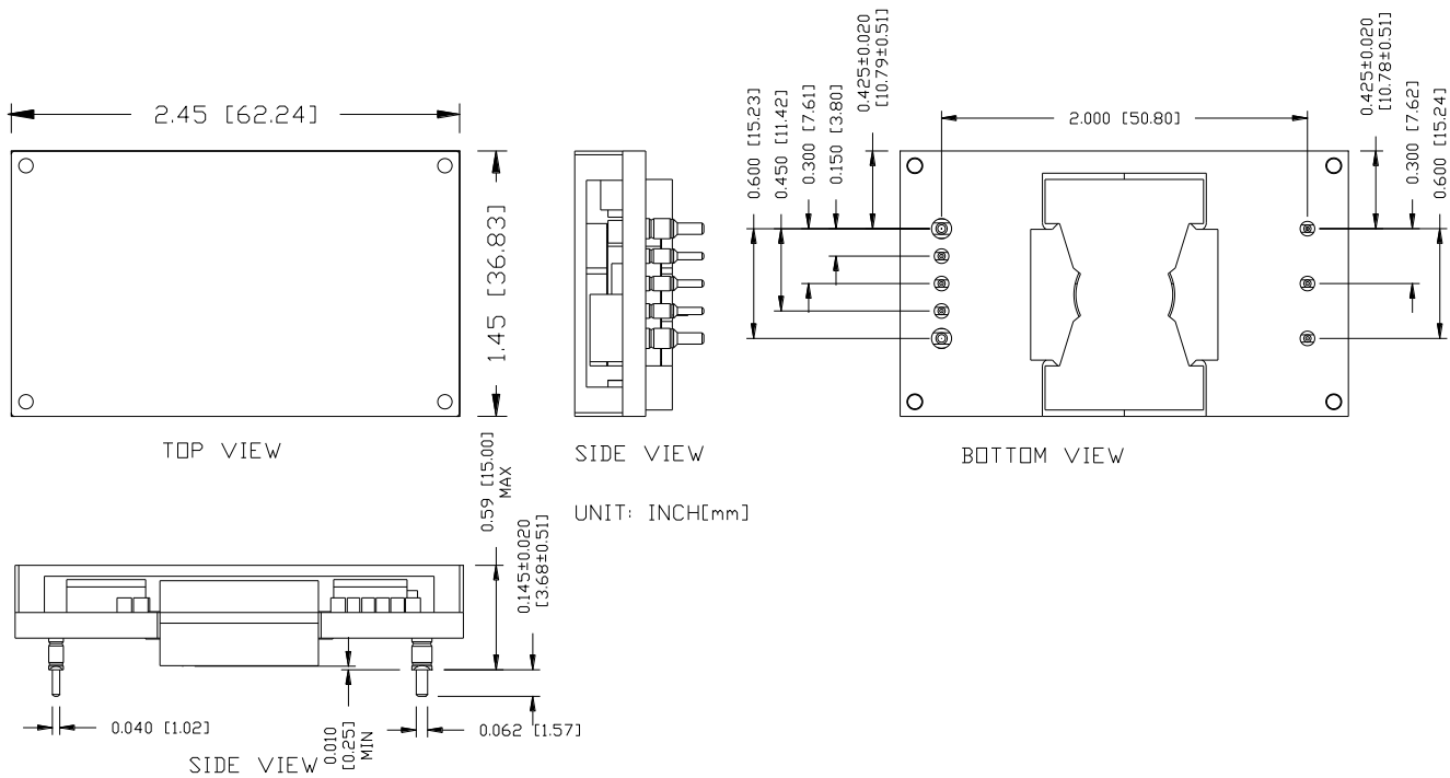
Figure 22. Outline
