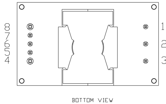
Figure 23. Pins
