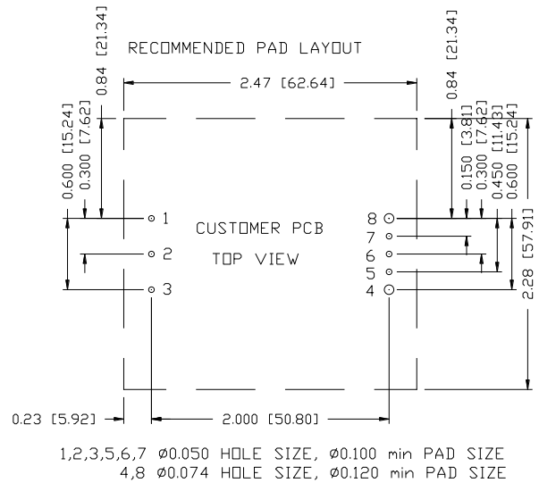
Figure 48. 0RQB-C5W24S Recommended pad layout-2
