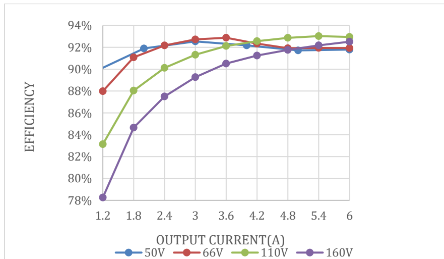
Figure 1. Efficiency data
