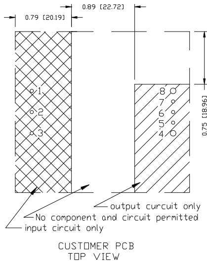
Figure 47. 0RQB-C5W24S Recommended pad layout-1
