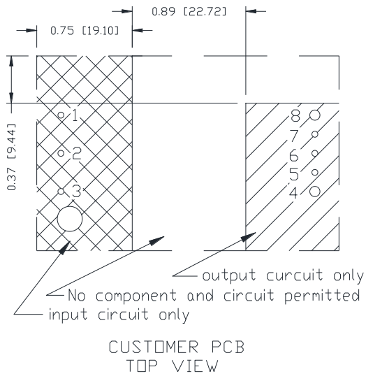
Figure 35. 0RQB-C5W240/L Recommended pad layout-1
