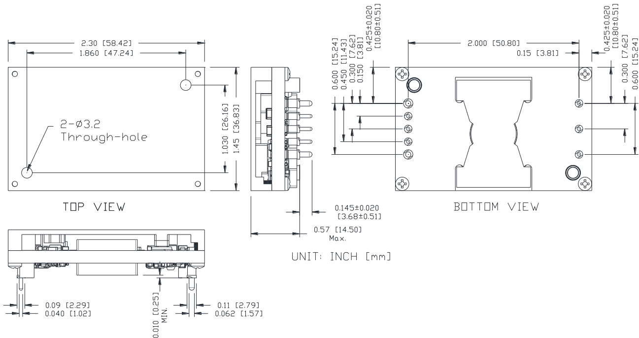
Figure 33. 0RQB-C5W240/L Outline
