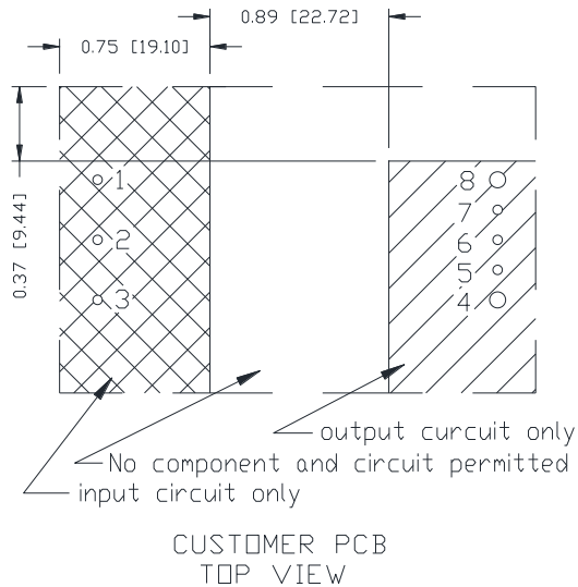
Figure 39. 0RQB-C5W24B Recommended pad layout -1
