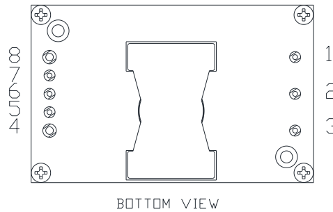
Figure 34. 0RQB-C5W240/L Pins
