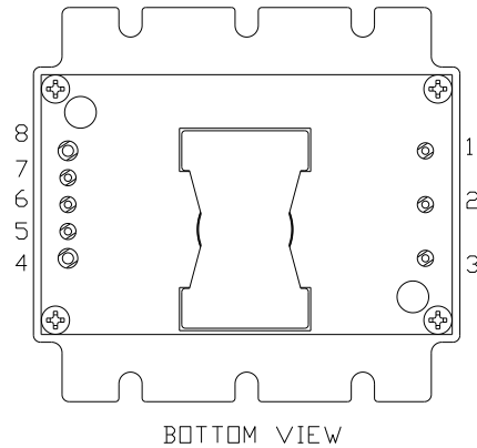
Figure 46. 0RQB-C5W24S Pins
