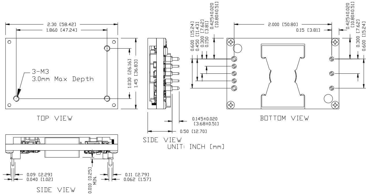
Figure 37. 0RQB-C5W24B Outline
