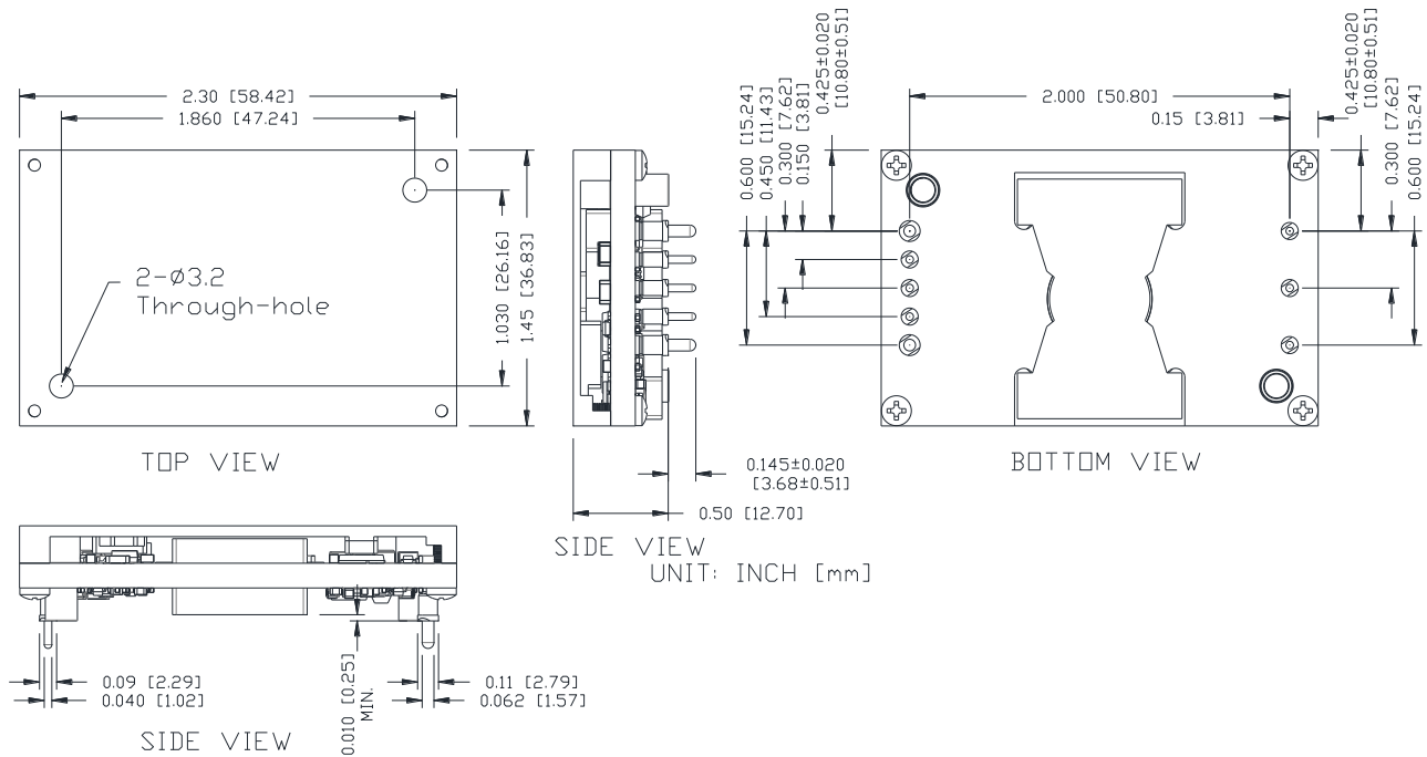
Figure 41. 0RQB-C5W24R Outline
