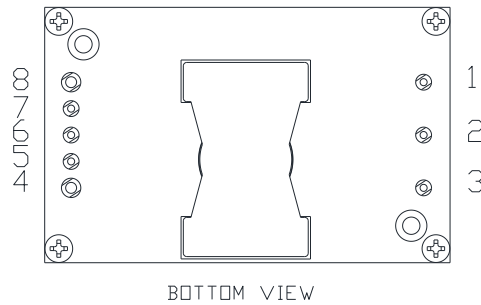
Figure 42. 0RQB-C5W24R Pins
