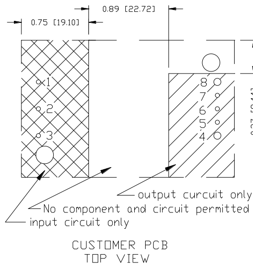
Figure 43. 0RQB-C5W24R Recommended pad layout-1
