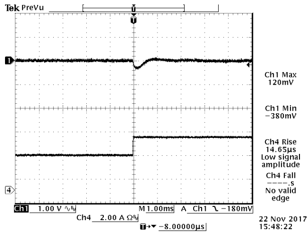
Figure 18. 10. Transient response 50% -75%
