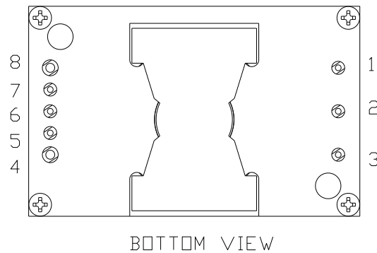
Figure 38. 0RQB-C5W24B Pins
