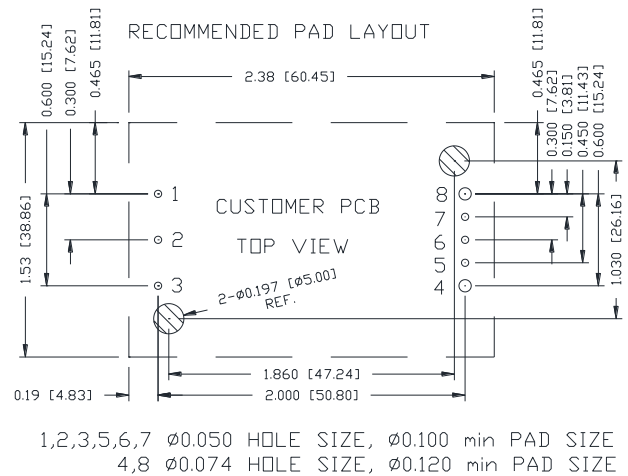
Figure 36. 0RQB-C5W240/L Recommended pad layout-2
