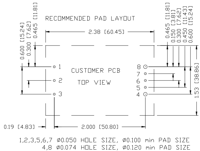
Figure 40. 0RQB-C5W24B Recommended pad layout -2
