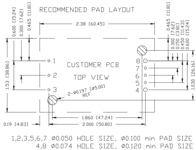
Figure 44. 0RQB-C5W24R Recommended pad layout-2
