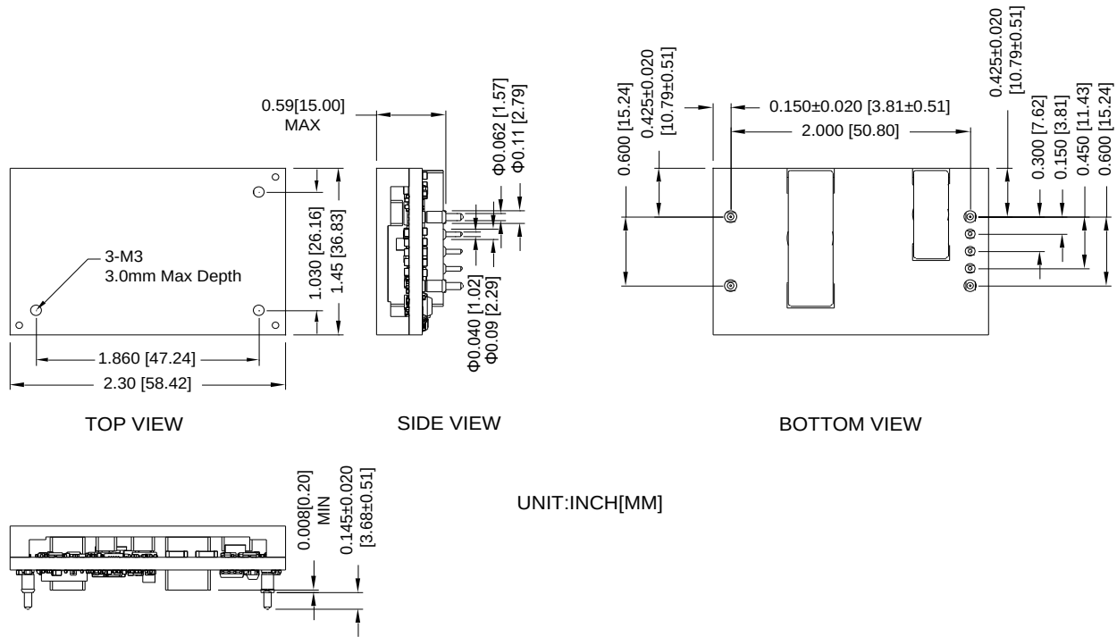
Figure 52. 0RQB-50Y05L/0 Outline
