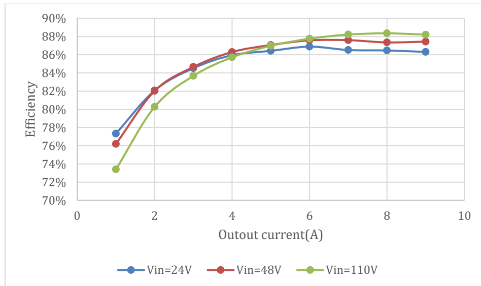
Figure 1. Efficiency data
