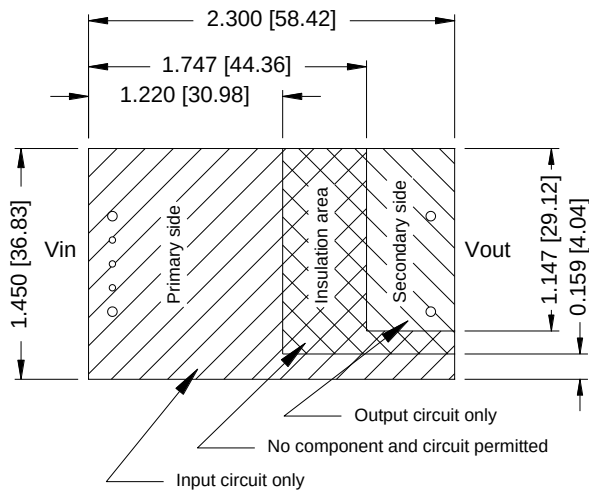
Figure 54. 0RQB-50Y05L/0 Recommended pad layout-1
