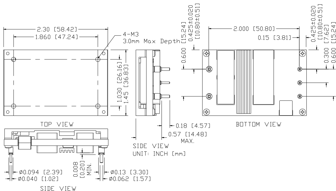
Figure 30. 0RQ1-H0T12A/B Outline
