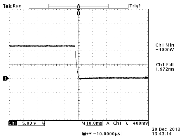
Figure 19. V_{out} = 12\text{ V} / 50\text{ A} @ V_{in} = 48\text{ V} , T_a = 25^\circ\text{C} , C_{ext} = 10000\text{ }\mu\text{F}
