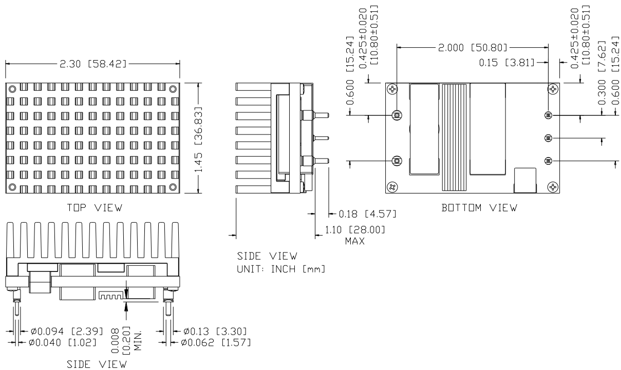
Figure 31. 0RQ1-H0T12C/D Outline
