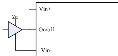
Figure 3. Control with open collector/drain circuit
