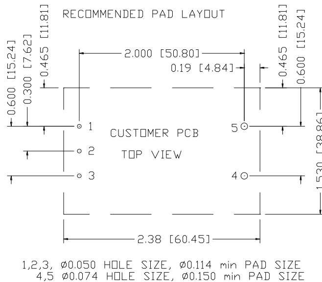
Figure 33. Recommended pad layout
