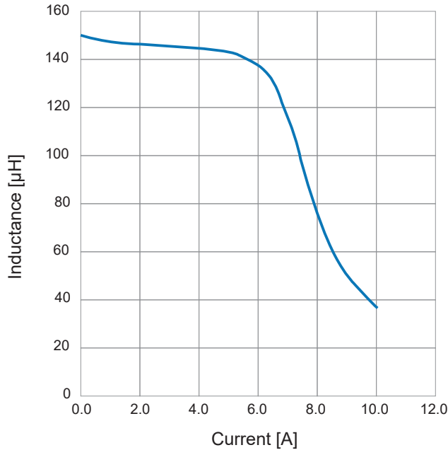
SPFC-EFD30-250
