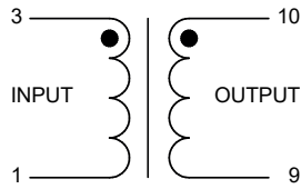
SPFC-EE20
