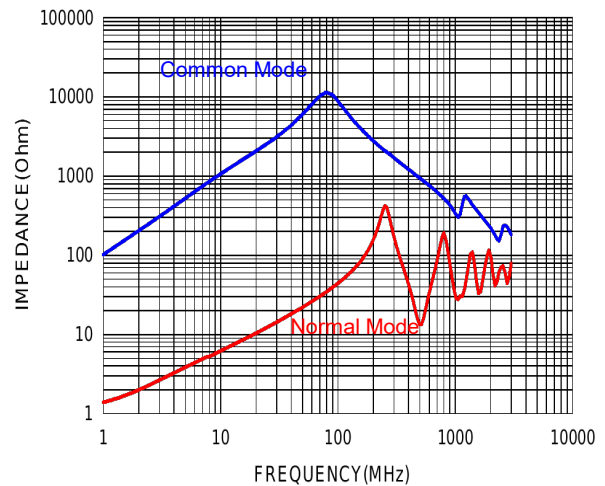
SPDL4532-220-2P-T
