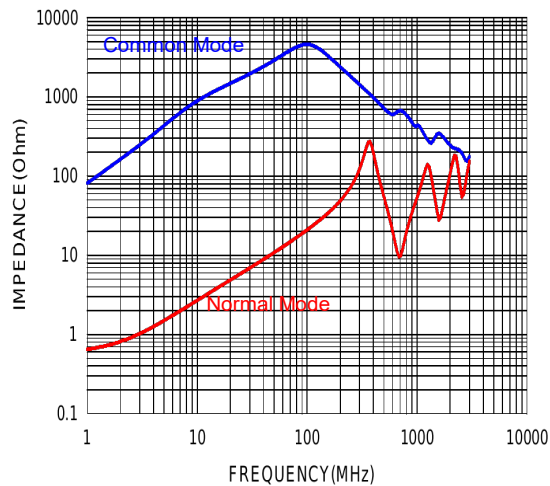
SPDL4532-110-2P-T
