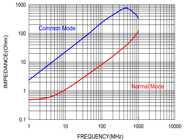
SPDL3216-221-2P-T
