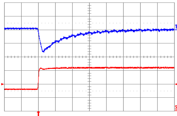
Fig. 1.2V.7: Output voltage response for V_{out} = 1.2 V to positive load current step change from 8 A to 16 A with slew rate of 5\ \text{A}/\mu\text{s} at V_{in} = 5 V. Top trace: output voltage (100 mV/div.); Bottom trace: load current (5 A/div.). C_o = 100\ \mu\text{F} ceramic. Time scale: 20 \mu\text{s} /div
