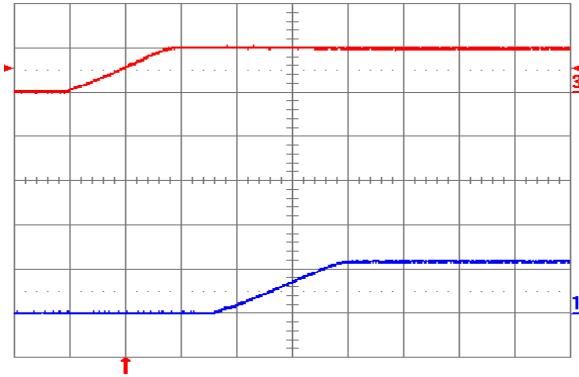
Fig. 1.2V.5: Turn-on transient for V_{out} = 1.2 V with application of V_{in} at full rated load current (resistive) and 100\ \mu\text{F} external capacitance at V_{in} = 5 V. Top trace: V_{in} (5 V/div.); Bottom trace: output voltage (1 V/div.); Time scale: 2 ms/div.
