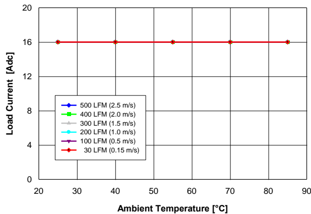
Fig. 1.8V.1: Available load current vs. ambient temperature and airflow rates for V_{out} = 1.8 V converter mounted vertically with V_{in} = 5 V, and maximum MOSFET temperature \leq 120 °C.
