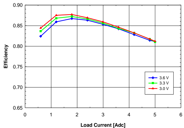
Fig. 0.7525V.4: Efficiency vs. load current and input voltage for V_{out} = 0.7525\text{ V} converter mounted horizontally with air flowing from pin 5 to pin 1 at a rate of 200 LFM (1 m/s) and T_a = 25\text{ }^{\circ}\text{C} .
