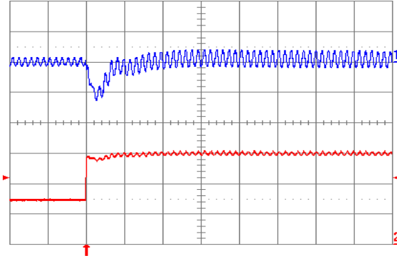
Fig. 1.8V.7: Output voltage response for V_{out} = 1.8V to positive load current step change from 2.5 A to 5 A with slew rate of 5 A/ \mu s at V_{in} = 5V . Top trace: output voltage (100 mV/div.); Bottom trace: load current (2 A/div.). C_o = 47 \mu F ceramic + 1 \mu F ceramic. Time scale: 20 \mu s/div.
