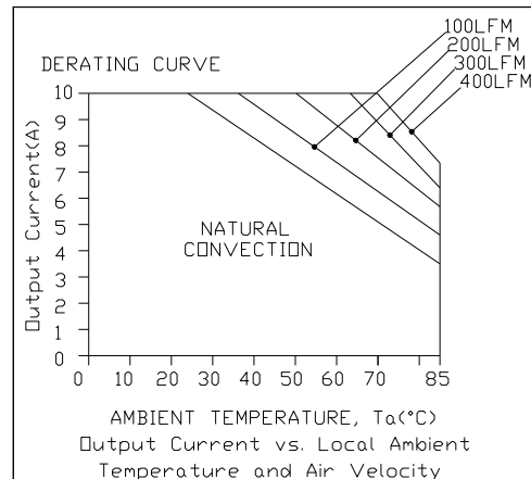
Figure 3. V_{in}=12\text{ V} , V_{out} = 2.5\text{ V}
